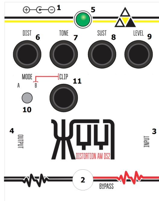
Figure 1: Pedal Unit Controls & I/O Elements
